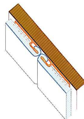
3 joint vertical
